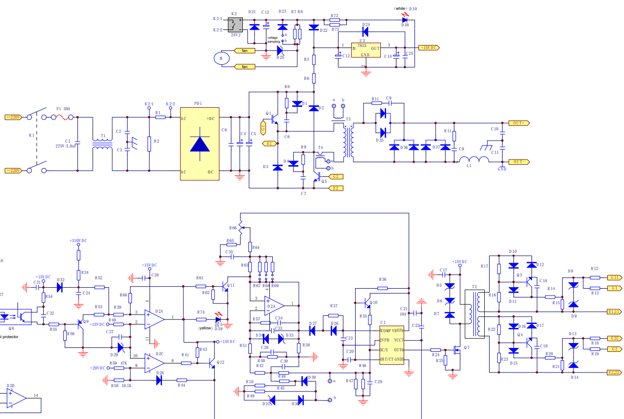
AW97117,AW9711C,AW97121 ELECTRIC CIRCUIT DIAGRAM Size A3 Number Revision Date: Sheet: 01 Drawn by: EZZ
